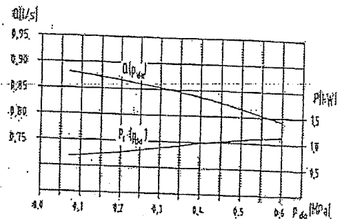
DIAGRAM p_{do}-Q, p_{s man}-P EQP-16-6 (230 V)
